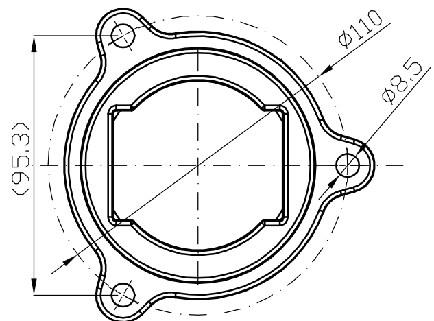
Bearing Housing
