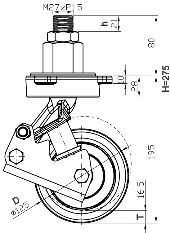
Stabilizing Caster
