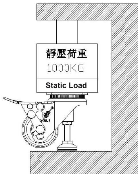
支撑脚静压荷重 Static Load with Foot
