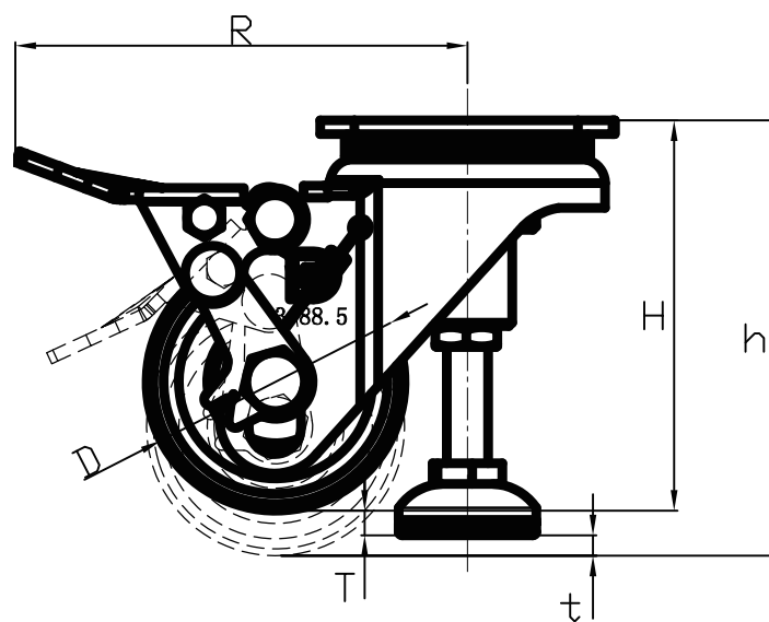
支撑升降脚轮 Levelling Caster
