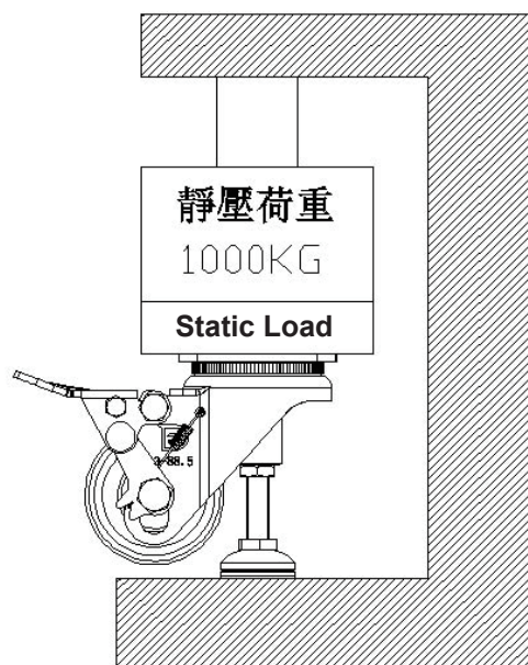
支撐腳靜壓荷重 Static Load with Foot
