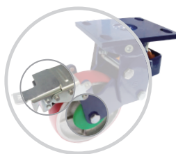
AK煞 Swivel W/Center Lock(AK type) &輪子可附塑膠防塵蓋(供選擇) Plastic Thread Guard(optional)
