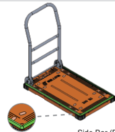
Side Bar (For DS-5 only)
